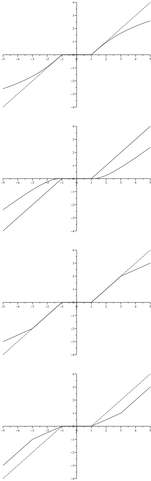
Figure 1: Graph of the proximal threshold \text{prox}_{\phi} , where \phi is as in (13) with \omega = 1 . The dashed line represents the usual soft threshold obtained with \psi = 0 . From top to bottom: (a) \psi = 0.05|\cdot|^4 ; (b) \psi = 0.9|\cdot|^{4/3} ; (c) \psi = d_{[-2,2]}^2/2 ; (d)
