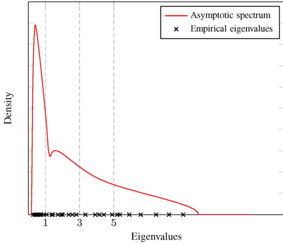
Fig. 2. Empirical and asymptotic eigenvalue distribution of \hat{\mathbf{R}}_N for L = 3 , \rho_1 = 1 , \rho_2 = 3 , \rho_3 = 5 , N/M = c = 3/8 , N = 30 , N_1 = N_2 = N_3 = 10 . In this case, there is only one cluster in the limiting eigenvalue distribution while there are 3 underlying eigenvalues to be estimated: The separability assumption does not hold true any more.
