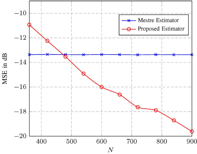
Fig. 4. Experienced MSE with N when \frac{N}{M} = \frac{3}{8} and (\rho_1, \rho_2, \rho_3) = (1, 2, 3) .
