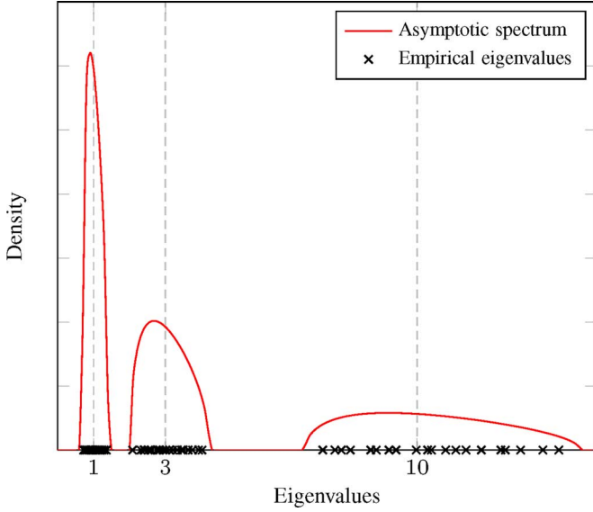
Fig. 1. Empirical and asymptotic eigenvalue distribution of \hat{\mathbf{R}}_N for L = 3 , \rho_1 = 1 , \rho_2 = 3 , \rho_3 = 10 , N/M = c = 0.1 , N = 60 , N_1 = N_2 = N_3 = 20 . In this case, there are 3 clusters in the limiting eigenvalues distribution and the separability assumption holds true.
