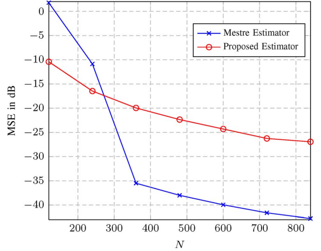
Fig. 3. Experienced MSE with N when \frac{N}{M} = \frac{3}{20} and (\rho_1, \rho_2, \rho_3) = (1, 3, 7) .
