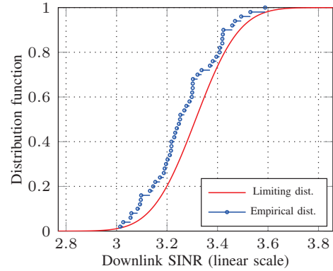
Figure 1. Simulation results for the empirical distributions of the downlink SINRs \{s_i\}_{i=1}^K (top) and uplink SINRs \{v_i\}_{i=1}^K (bottom), compared to the limiting expressions given by Theorem 1. The empirical distribution is evaluated for a single generation of the random matrix \mathbf{X} . Both graphs are drawn for N = 200 , K = 50 , \sigma^2 = 1 , and \alpha = \sigma^2/c .
