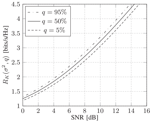
Figure 2. Asymptotic values for quantiles q = 0.05, 0.5, 0.95 of the users' rates in a MAC channel given by Corollary 1, versus the signal-to-noise ratio (SNR) 1/\sigma^2 . Here, N = 200 and K = 50 .
