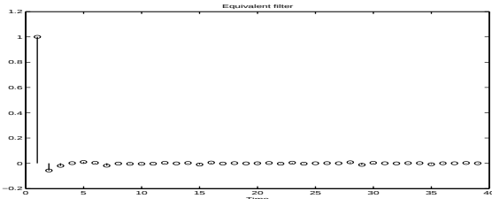
Figure 2: Equivalent impulse response f for experiment 1.
