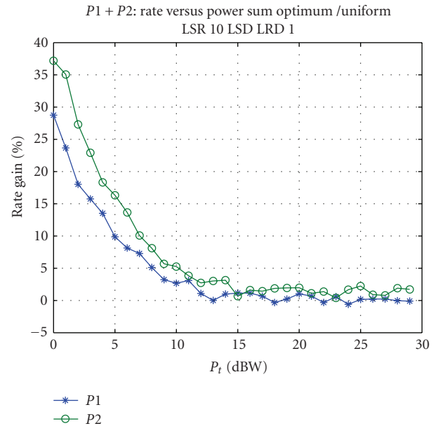
FIGURE 8: Rate gain with the optimized power allocation compared to the uniform one, versus P_t (dBW) for the two protocols and the sum power constraint. Taps of the |\lambda_{sr}(k)|^2 have a variance 10 dBs above those associated with the |\lambda_{sd}(k)|^2 and the |\lambda_{rd}(k)|^2 .
