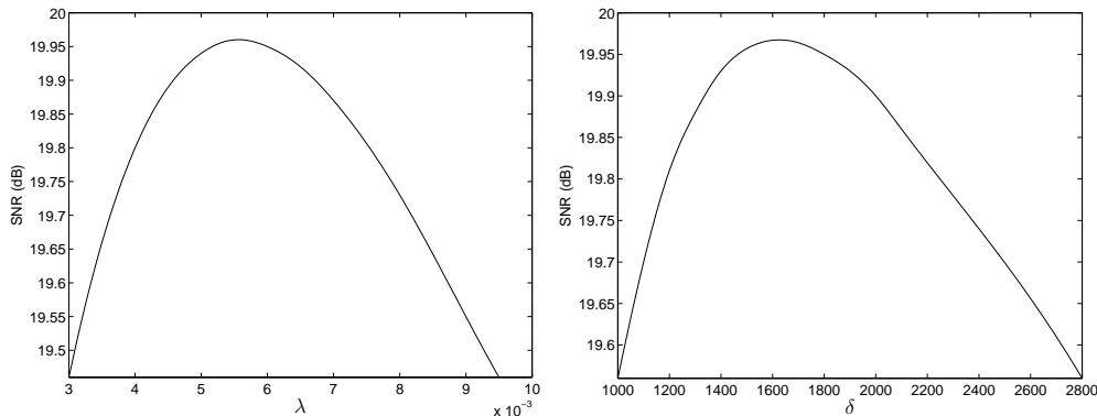
Figure 3: SNR vs \lambda when \delta = 1700 (left) and SNR vs \delta when \lambda = 6 \times 10^{-3} (right) for slice No 82 using Poly1 sampling, 3MG algorithm and \ell_2 - \ell_1 regularization.
